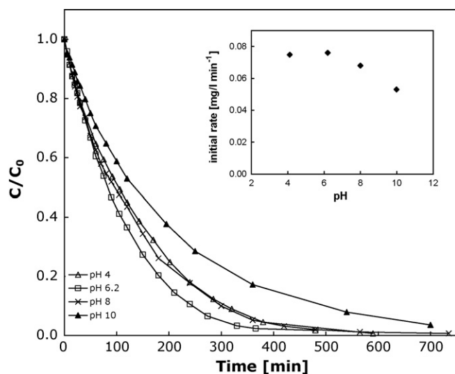
Fig. 8. Bleaching of RNO in the photocatalytic reactor with \text{TiO}_2 coated liner in air saturated solution at different pH. Inset graph: initial rate of bleaching of RNO as a function of pH.
